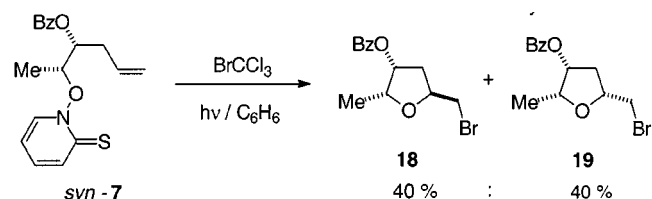
Scheme 5. Preparation of tetrahydrofurans 18 and 19 from syn - 7
