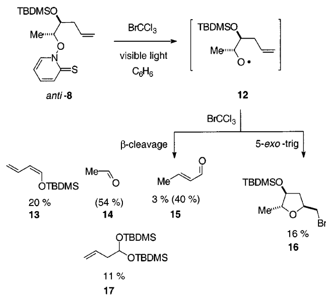
Scheme 4. Photolysis of TBDMS-protected alkoxy radical precursor anti - 8 in the presence of \text{BrCCl}_3 ; Figures in parentheses denote yields of volatile aldehydes as derived from a separate NMR experiment in \text{C}_6\text{D}_6 .
