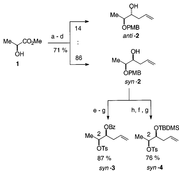
Scheme 1. Synthesis of tosylates syn-3–4 ; reagents and conditions: (a) NaH, p -methoxybenzyl chloride (PMBCl), DMF (75%); (b) DI-BAH, Et 2 O, –78 °C; (c) allyl magnesium bromide, Et 2 O, –78 °C (94% step b and c); (d) column chromatography, SiO 2 , petroleum ether/CH 2 Cl 2 /MeOH, 10/4/1(v/v/v); (e) PhCOCl, DABCO, CH 2 Cl 2 (99%); (f) DDQ, H 2 O/CH 2 Cl 2 (94%) [84%]; (g) TosCl, DABCO, CH 2 Cl 2 (94%) [96%]; (h) ( tert -butyl)dimethylsilyl chloride, imidazole, DMF (94%); yields in square brackets refer to the synthesis of syn-4
