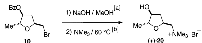
Scheme 6. Synthesis of (+)- allo -muscarine (+)- 20 : (a) 76% yield; (b) 38% yield and 60% of recovered starting material
