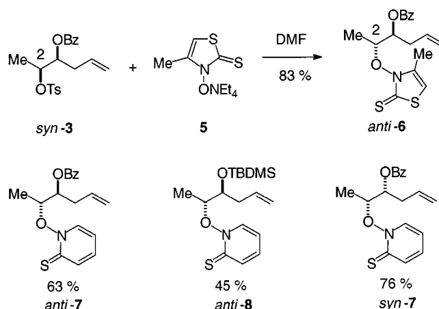
Scheme 2. Preparation of alkoxyl radical precursors 6–8
